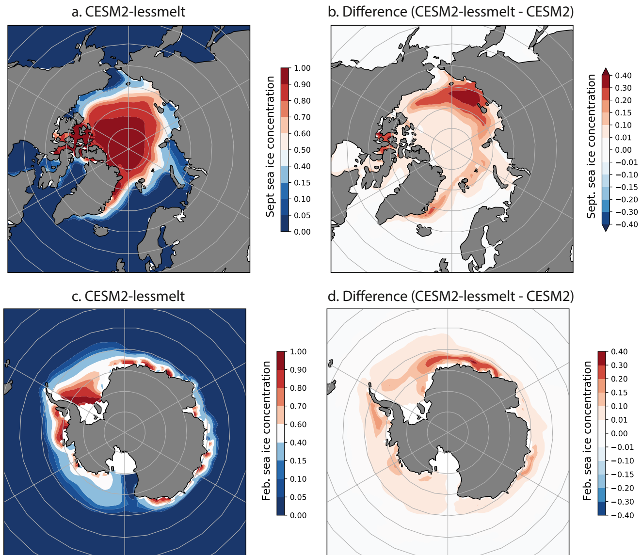
Figure 2. Late summer sea ice concentration in preindustrial control runs: (a) September Arctic CSM2-lessmelt, (b) Difference September Arctic (CESM2-lessmelt—CESM2), (c) February Antarctic CSM2-lessmelt, and (d) Difference February Antarctic (CESM2-lessmelt—CESM2). Values are overlapping 200-year averages as in Figure 1. Note: Nonlinear color scale used to emphasize low ice concentrations.
