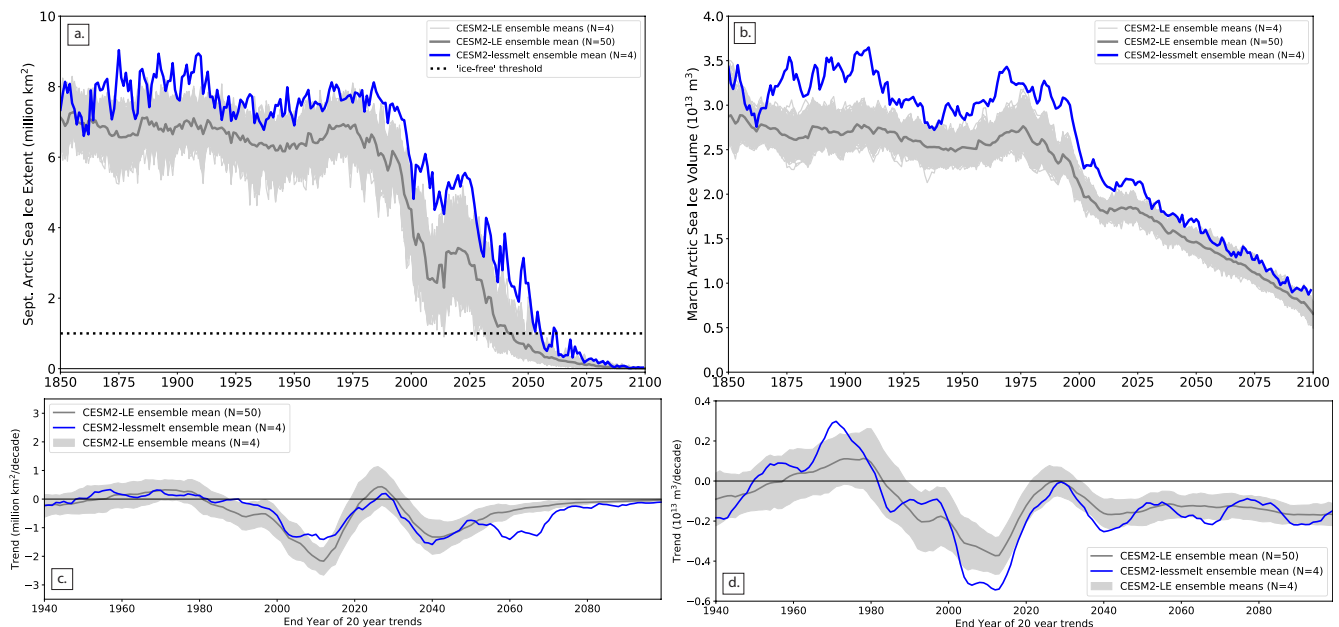
Figure 12. CSM2-LE and CSM2-lessmelt Arctic sea ice: (a) September extent ensemble mean 1850–2100 timeseries, (b) March volume ensemble mean 1850–2100 timeseries, (c) September extent ensemble mean 20-year trends, (d) March volume ensemble mean trends. Gray shading shows 95% confidence intervals on trends calculated by bootstrapping CSM2-LE ensemble means with four members 1,000 times.
