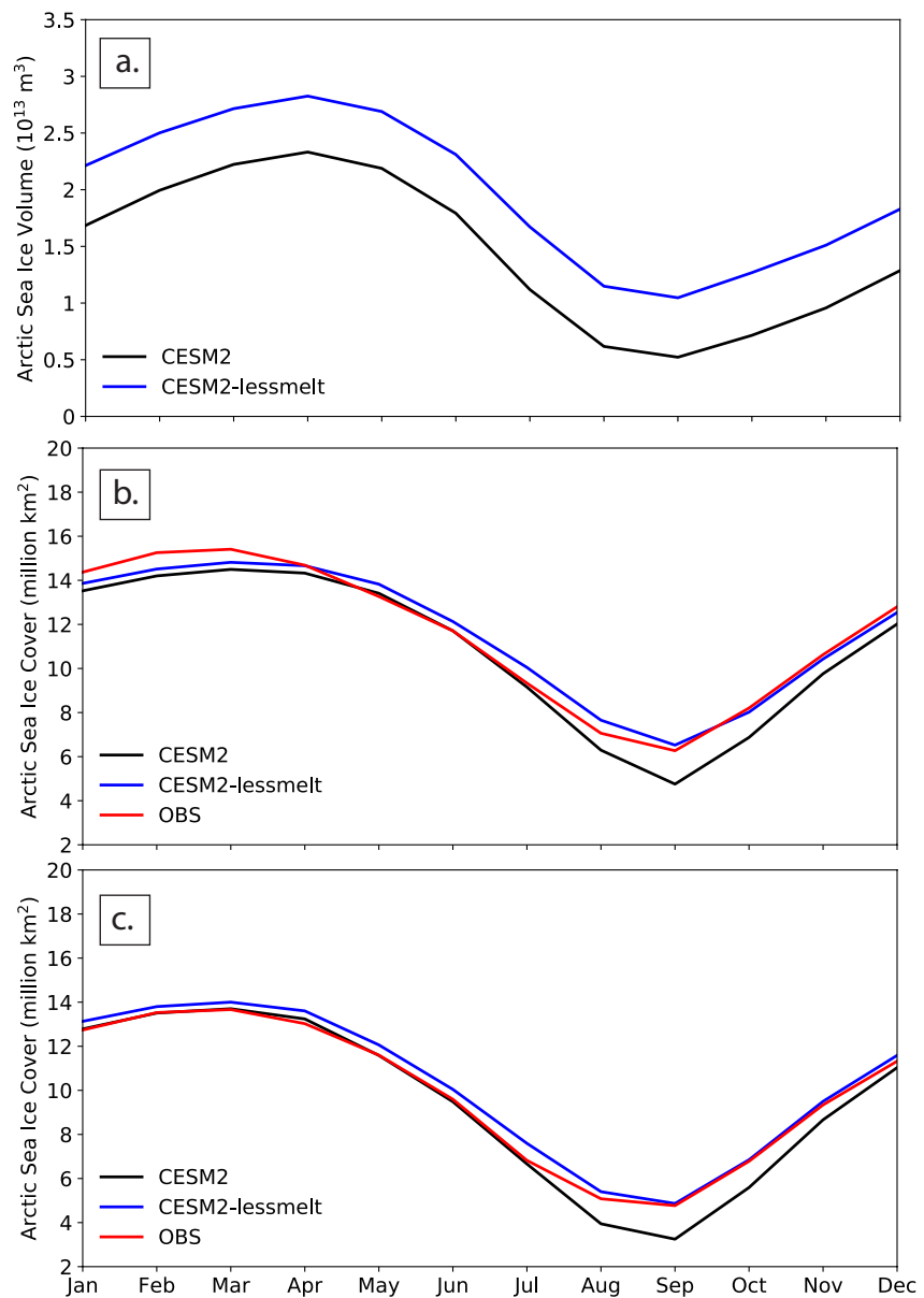
Figure 8. Present-day (1979–2014) ensemble mean seasonal cycle in CSM2-LE and CSM2-lessmelt: (a) Arctic sea ice volume, (b) Arctic sea ice extent, and (c) Arctic sea ice area. Observations are from NSIDC sea ice index with pole filling (Fetterer et al., 2017).
