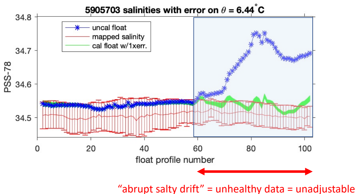
Figure 6. WMO ID 5905703, DAC = AOML/SIO. An example of "abrupt salty drift". Starting from cycle 59, float salinity data drifted salty abruptly and rapidly. There were large jumps between profiles and many reversals. Salinity data from cycle 59 onwards should be considered as bad and unadjustable.
