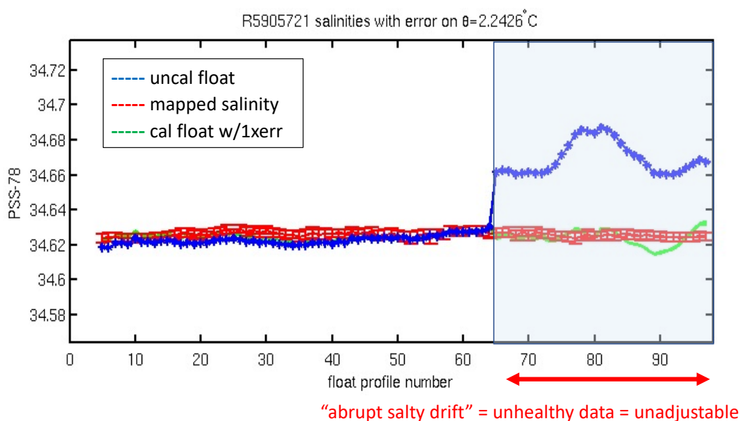
Figure 7. WMO ID 5905721, DAC = AOML/SIO. Another example of "abrupt salty drift". After cycle 65, salinity jumped salty by > 0.035 , with no consistent sensor trend after that. Therefore salinity data from cycle 65 onward should be considered as bad and unadjustable.
