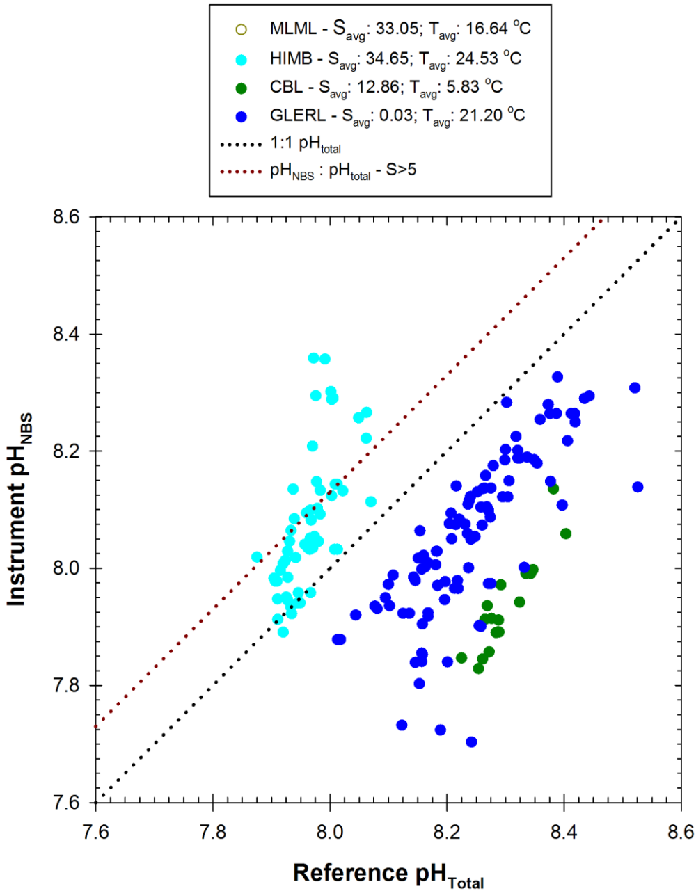
Figure 18 . Global response plot for Idronaut 305 Plus pH sensor observed during ACT field trials. Black dotted line represents 1:1 correspondence, dark red dotted line represents correspondence predicted based on difference between pH_{NBS} and pH_{Total} in seawater ( pH_{NBS} = pH_{Total} + 0.13 ).
