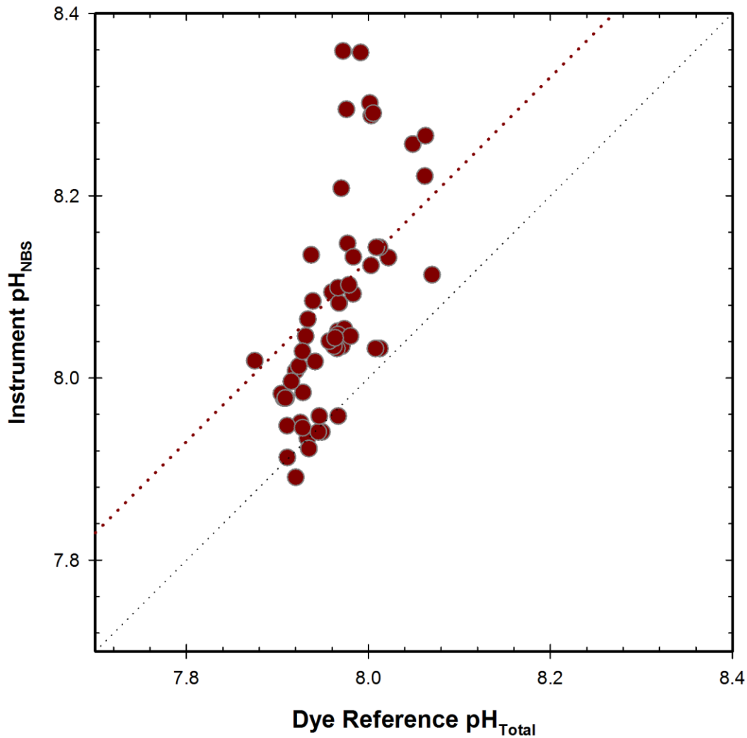
Figure 11. HIMB field response plot of the Idronaut 305 Plus pH sensor compared to reference pH Total samples. Fine dotted line represents 1:1 correspondence, coarse dotted line represents correspondence predicted based on difference between pH NBS and pH Total in seawater ( \text{pH}_{\text{NBS}} = \text{pH}_{\text{Total}} + 0.13 ).
