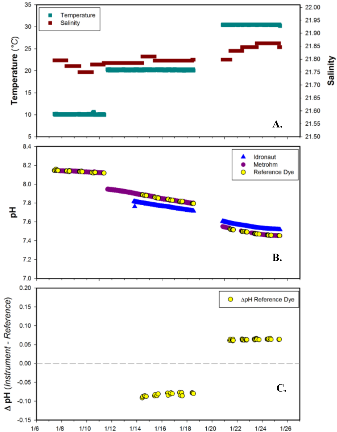
Figure 4. Time series results of the Idronaut 305 Plus pH sensor for the stable portion of the brackish water trials. Measurements taken during temperature and pH shifts have been removed. Panel (a) temperature and salinity conditions during the seawater trials; panel (b) measured pH from the CSI pH plotted against both Metrohm and Dye reference pH measurements; and, panel (c) the difference between Idronaut and reference pH values.
