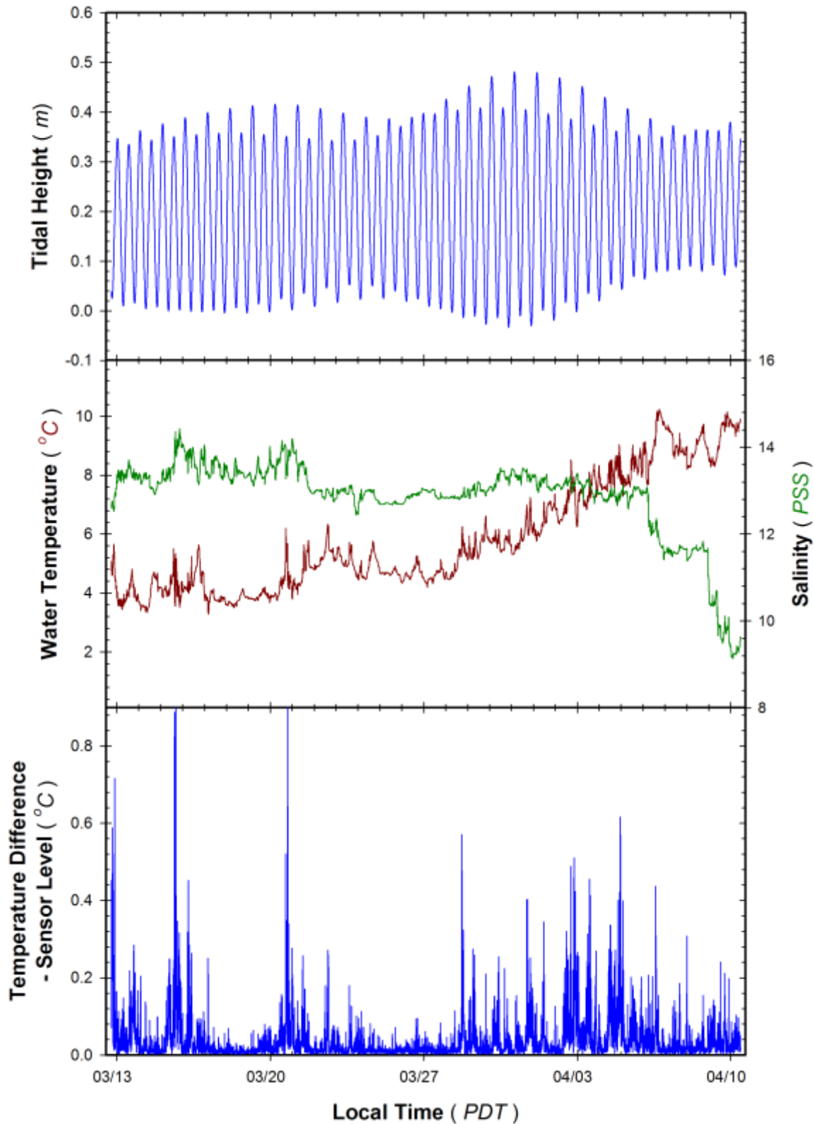
Figure 12. Environmental conditions encountered during the 1 month CBL floating dock deployment. Test sensor array deployed at 1 m fixed depth, variation in local tidal heights indicate active water flow around instrument ( Top Panel ). Variation in salinity (green) and temperature (red) at depth of instrument sensor detected by an SBE 26 and two RBR Solo thermistors ( Middle Panel ). Temperature range determined from max-min temperatures detected by RBR and SBE thermistors spanning instrument sensor array ( Bottom Panel ).
