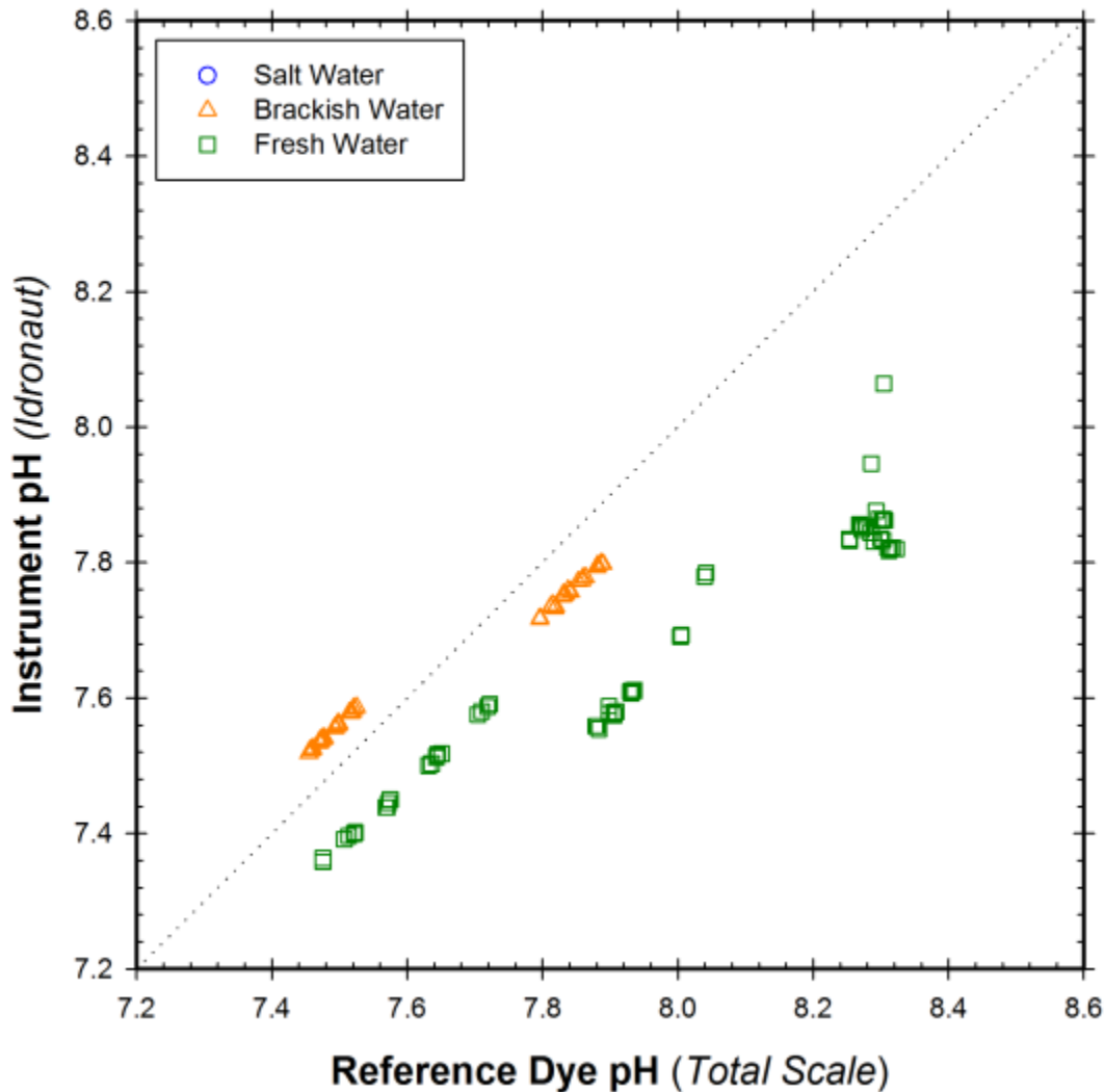
Figure 6. Cross plot of Idronaut 305 Plus pH sensor measurements against the dye reference pH measurements for 201 matched observations during the stable Temperature and Salinity portions of the entire lab test.
