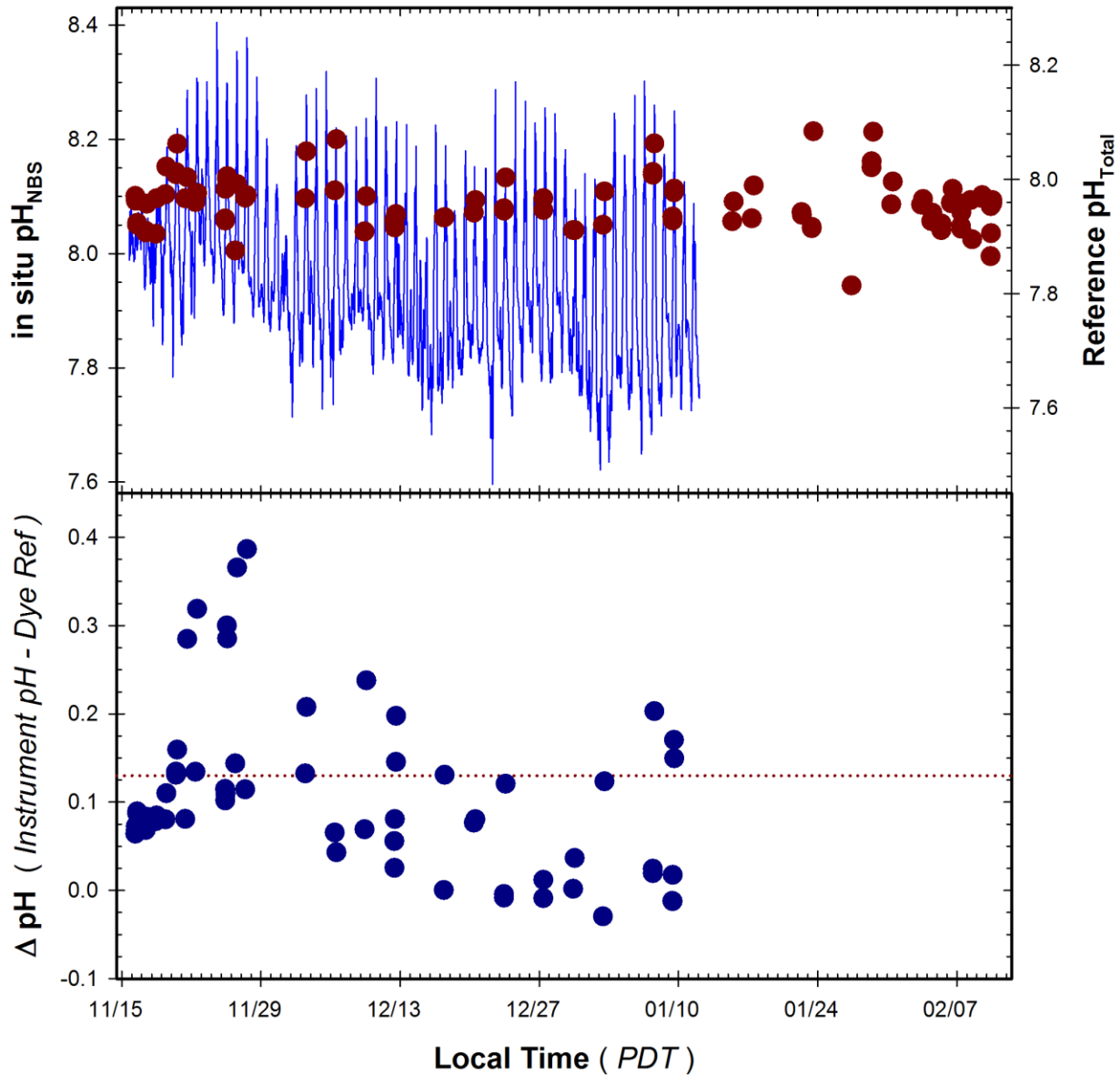
Figure 10. Time series of pH measured by the Idronaut 305 Plus pH sensor during the 3 month HIMB trial. Top Panel: Continuous \text{pH}_{\text{NBS}} recordings from instrument (blue line) and \text{pH}_{\text{Total}} of adjacent grab samples determined by mCP dye (red circles). Bottom Panel: Difference in measured pH relative to reference samples (Instrument – Dye Ref) observed during deployment. Dashed line represents offset (ca 0.13) predicted due to difference in \text{pH}_{\text{NBS}} and \text{pH}_{\text{Total}} scales used by the Idronaut pH sensor and the dye reference method.
