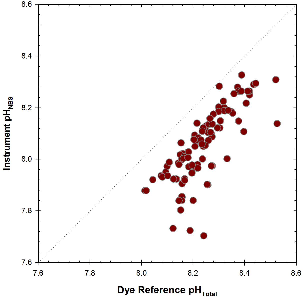
Figure 17. GLERL field response plot of Idronaut 305 Plus pH sensor compared to reference pH Total samples. Fine dotted line represents 1:1 correspondence.
