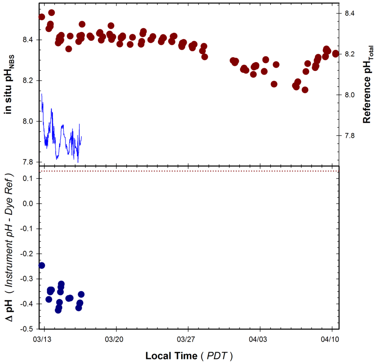
Figure 13. Time series of pH measured by Idronaut 305 Plus pH sensor deployed during the 1 month CBL trial. Top Panel: Continuous pH NBS recordings from instrument (blue line) and pH Total of adjacent grab samples determined by mCP dye (red circles). Bottom Panel: Difference in measured pH relative to reference samples (Instrument – Dye Ref) observed during deployment. Dashed line represent offset (ca 0.13) predicted due to difference in pH NBS and pH Total scales used by the Idronaut sensor and the dye reference method.
