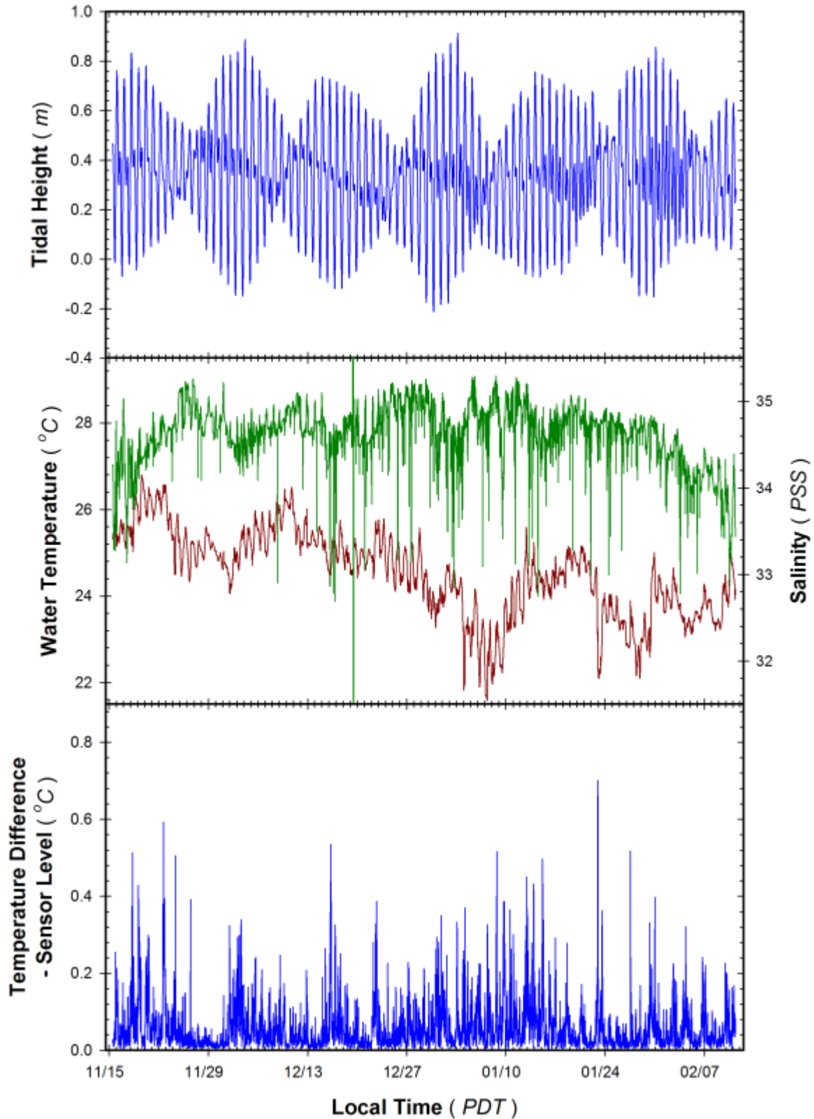
Figure 9. Environmental conditions encountered during the 3 month HIMB offshore deployment on the NOAA CRIMP Buoy. Test sensor array deployed at 1 m fixed depth, variation in local tidal heights indicate active water flow around instrument ( Top Panel ). Variation in salinity (green) and temperature (red) at depth of instrument sensor detected by an SBE 26 and two RBR Solo thermistors ( Middle Panel ). Temperature range determined from max-min temperatures detected by RBR and SBE thermistors spanning instrument sensor array ( Bottom Panel ). 29
