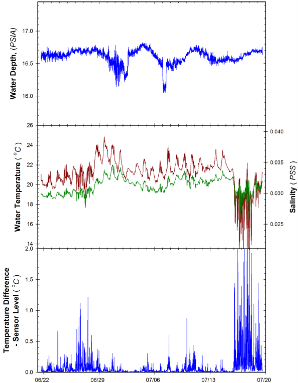
Figure 15. Environmental conditions encountered during the 1 month freshwater deployment adjacent to the NOAA GLERL Pier. Test sensor array deployed on bottom, variation in local water depth measured as PSIA by an SBE 26PLUS Wave gauge indicating active water flow around instrument ( Top Panel ). Variation in salinity (green) and temperature (red) at depth of instrument sensor detected by SBE 26 and two RBR Solo thermistors ( Middle Panel ). Temperature range determined from max-min temperatures detected by RBR and SBE thermistors spanning instrument sensor array ( Bottom Panel ). Storm event contributed to higher variation in environmental conditions near end of deployment period.
