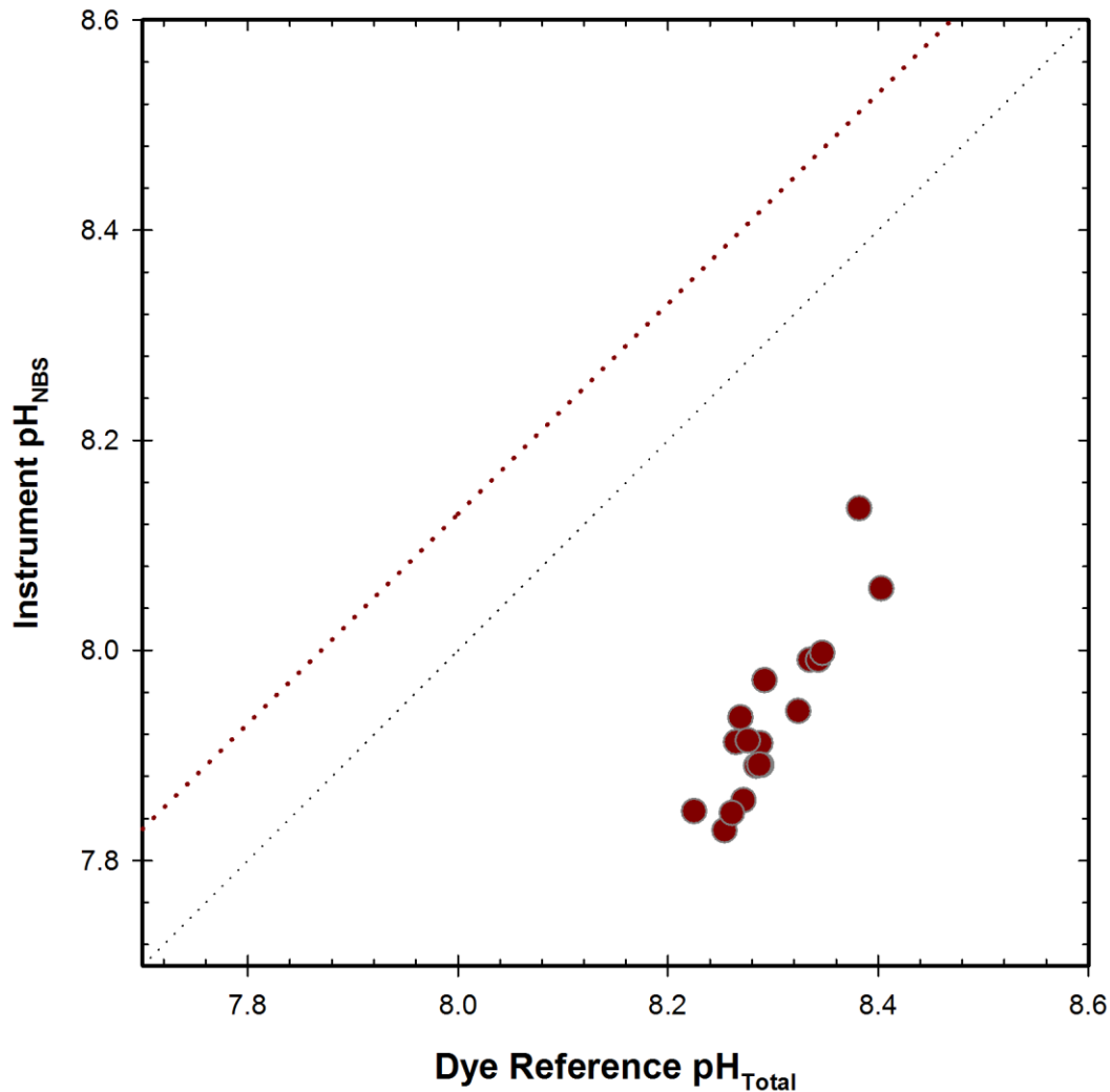
Figure 14. CBL field response plot of Idronaut 305 Plus pH sensor compared to reference pH Total samples. Fine dotted line represents 1:1 correspondence, coarse dotted line represents correspondence predicted based on difference between pH NBS and pH Total in seawater ( \text{pH}_{\text{NBS}} = \text{pH}_{\text{Total}} + 0.13 ).
