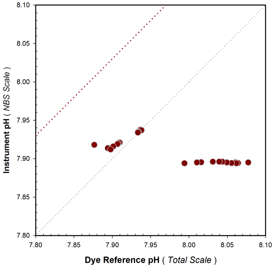
Figure 7. Cross plot of Idronaut 305 Plus pH sensor measurements against the dye reference pH measurements for 32 matched observations during the repeated seawater exposure that occurred on week ten of the laboratory test. Temperature was varied over the course of 3 days between 26 and 10 °C.
