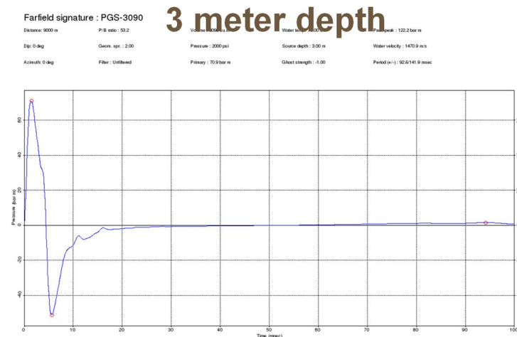
Figure 4: Farfield signature: PGS-3090; 3 m depth: Airgun signature in bar metres (bar m) (supplied by W Pramik, Geokinetics).
