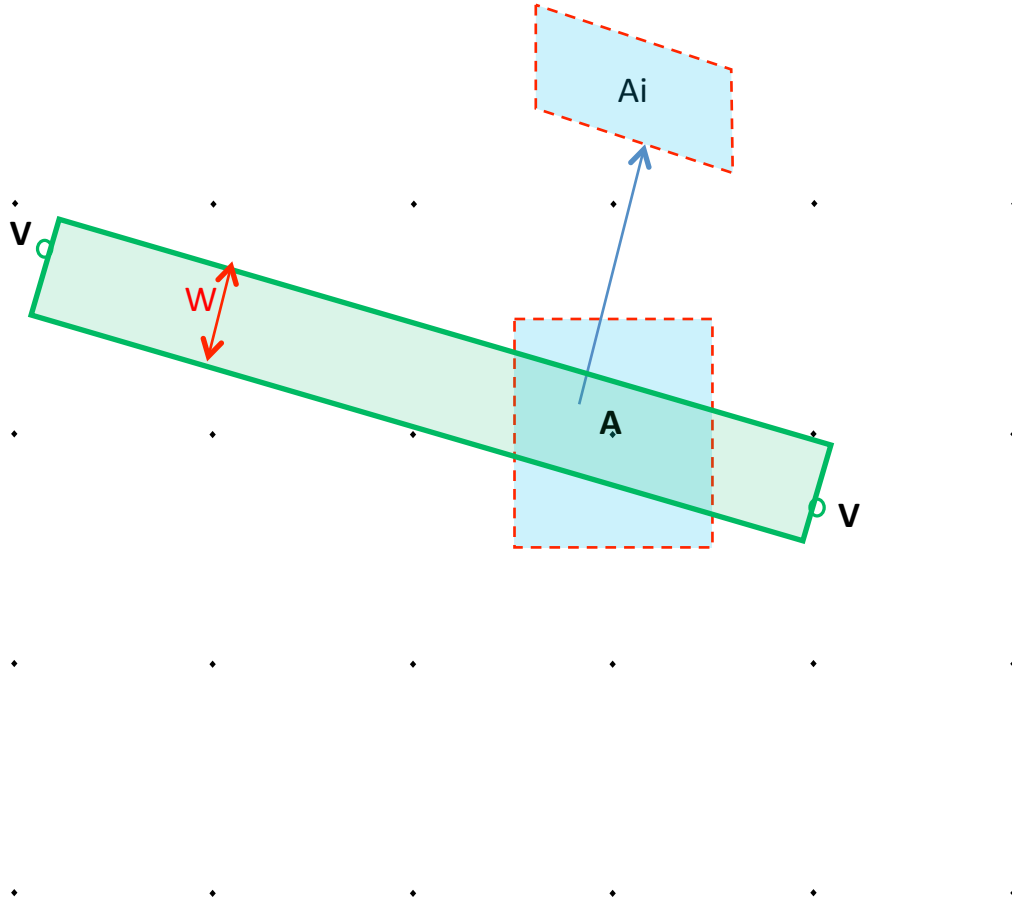
Figure 6-8: Application of Constraint Line - Uniformly-Sampled Terrain
