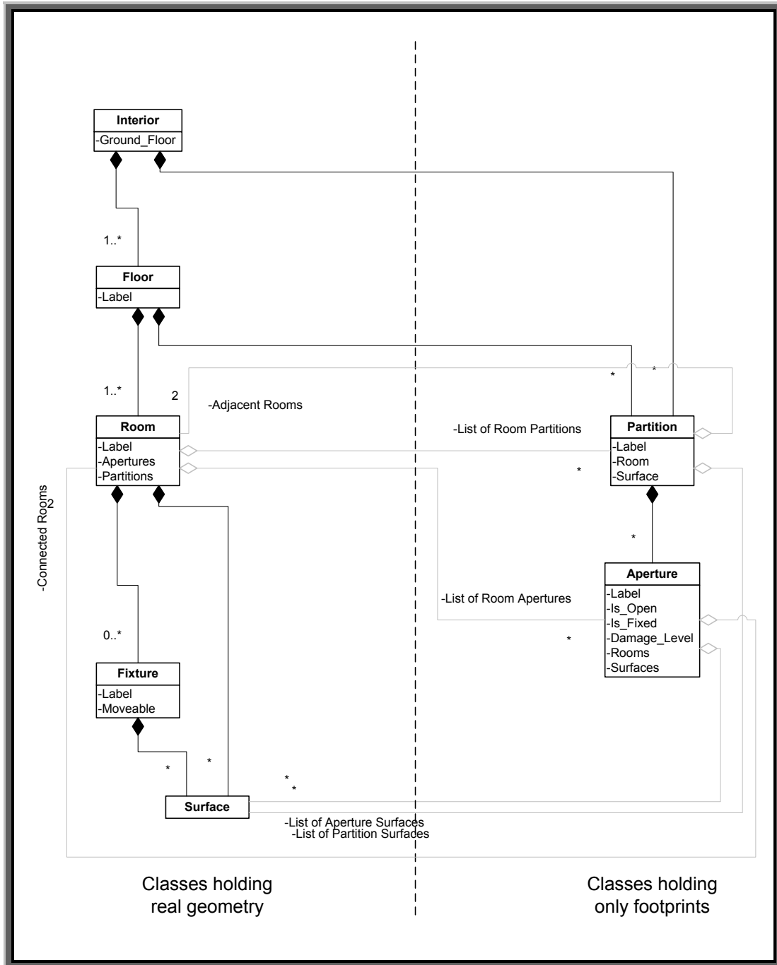
Figure 6-6: CDB Model Interior Object Model
