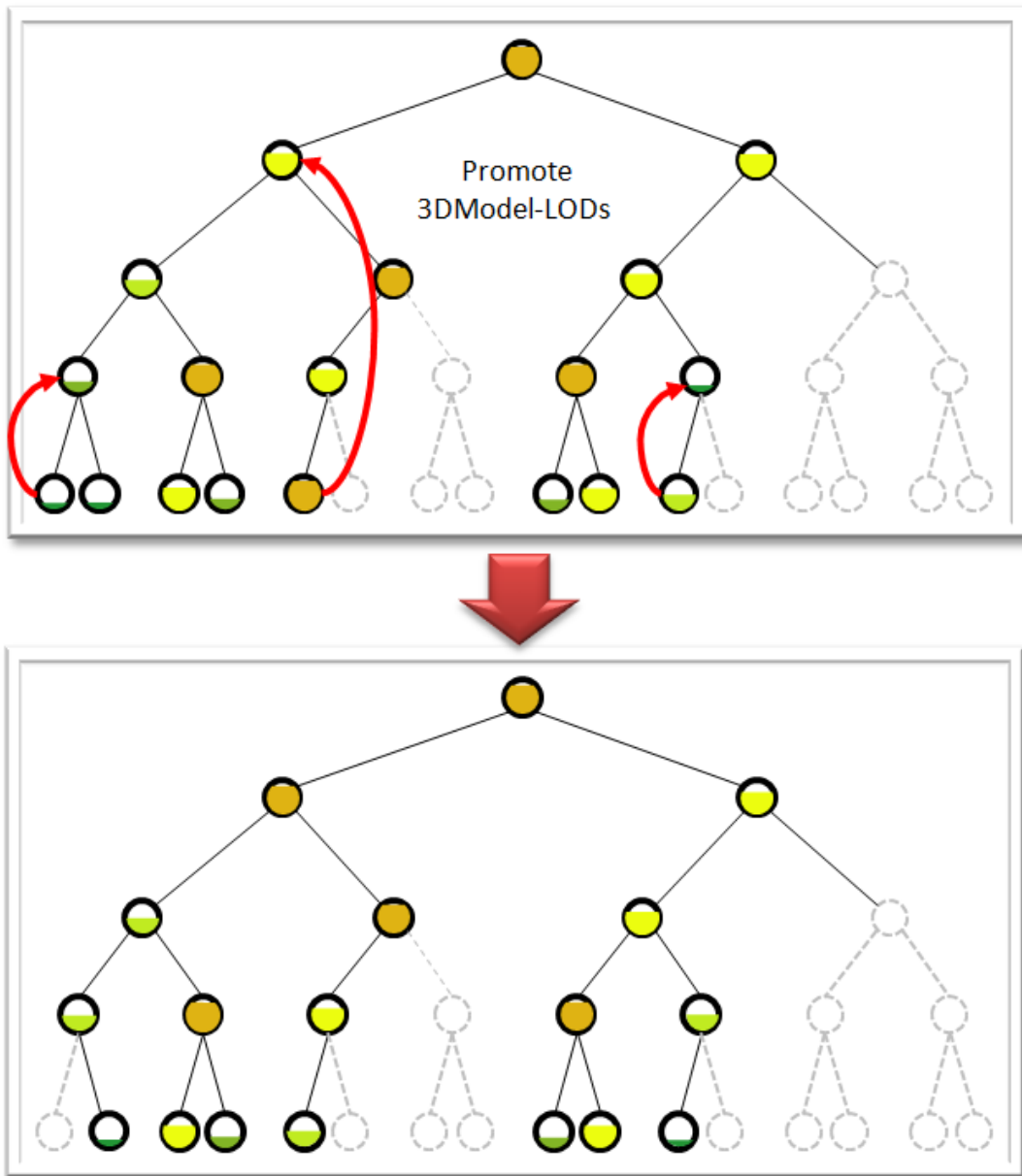
Figure 6-16: Compacting the GSModel Dataset
